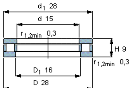
Complete bearing
