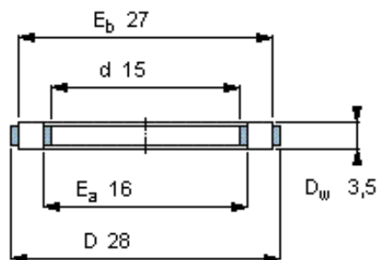
Roller and cage thrust assembly
